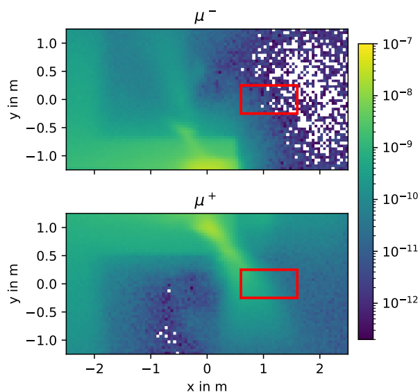
Figure 2: Simulated muon flux at the NaNu detector (red) without the NaNu MIB. Dominant component: \mu^+
